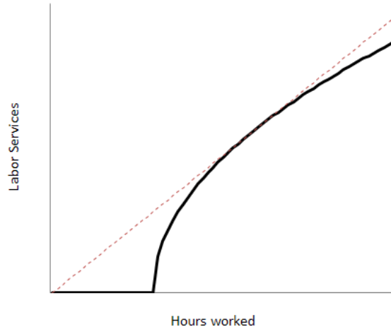
Figure 1: Nonlinear labor services mapping
